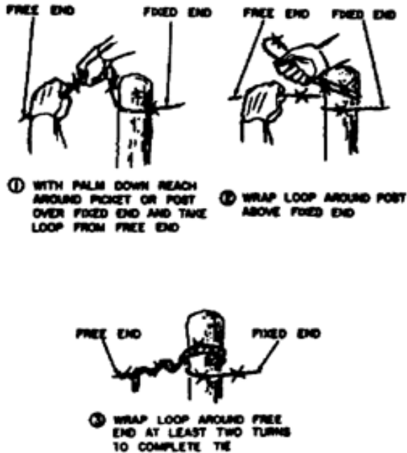
Figure 4-16. Post tie.
